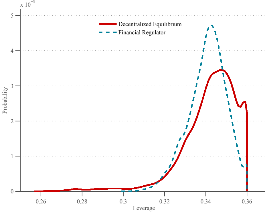
Figure 3: Ergodic Distribution of Leverage ( \frac{-b_{t+1} + \theta w_t h_t}{q_t K} )
